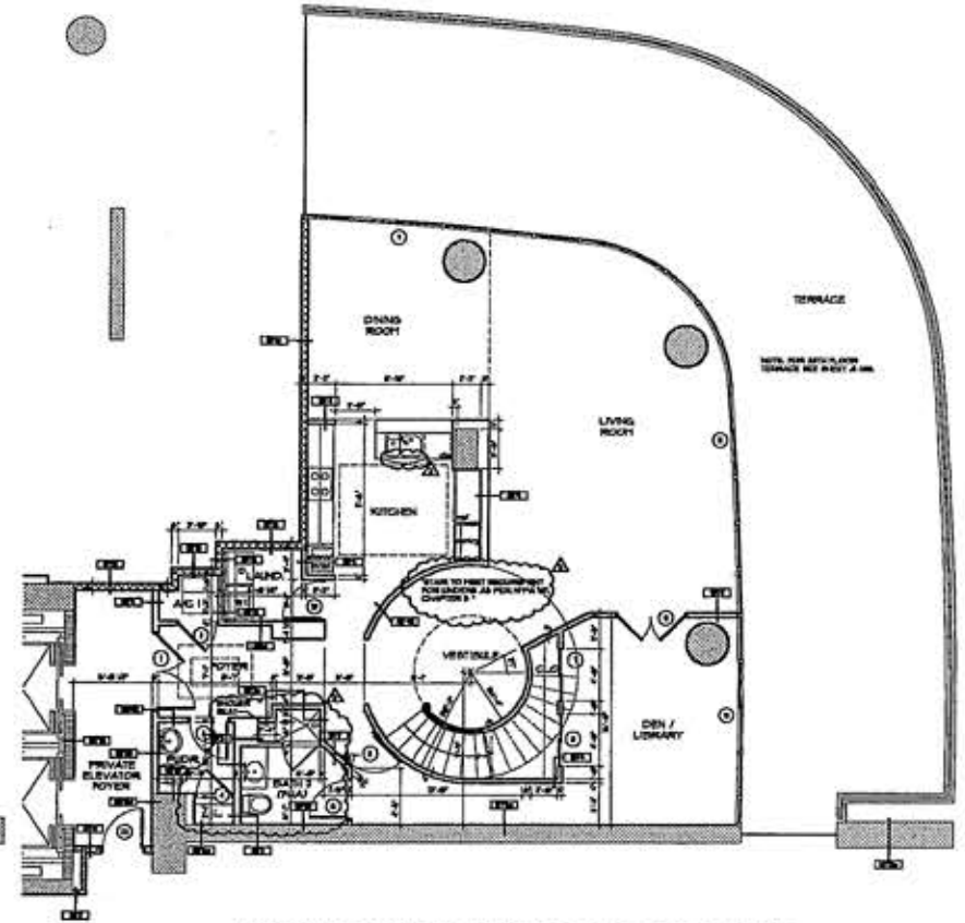
TYPICAL UNIT-19 LOWER LEVEL FLOOR PLAN (16TH FLOOR - SOUTH TOWER) (18TH FLOOR SIMILAR)
