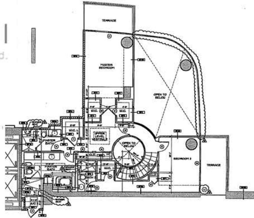
TYPICAL UNIT-19 UPPER LEVEL FLOOR PLAN (17TH AND 19TH FLOORS - SOUTH TOWER)
